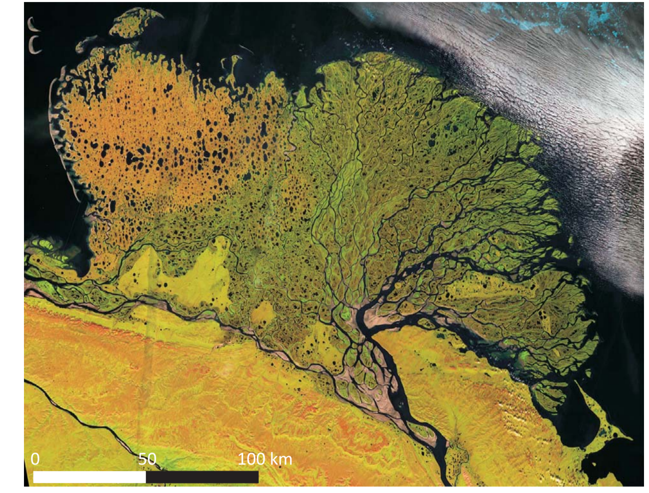
Fig. 2: Satellite image of the Lena Delta region, © ESA-BELSP0 2015, from 27 July 2014
